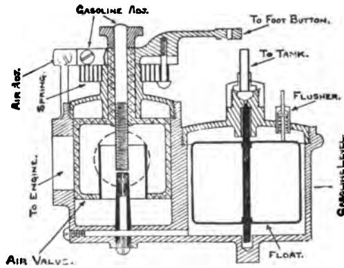
FIG. 418.—Section of the "Dyke" Float Feed Carburetter.
